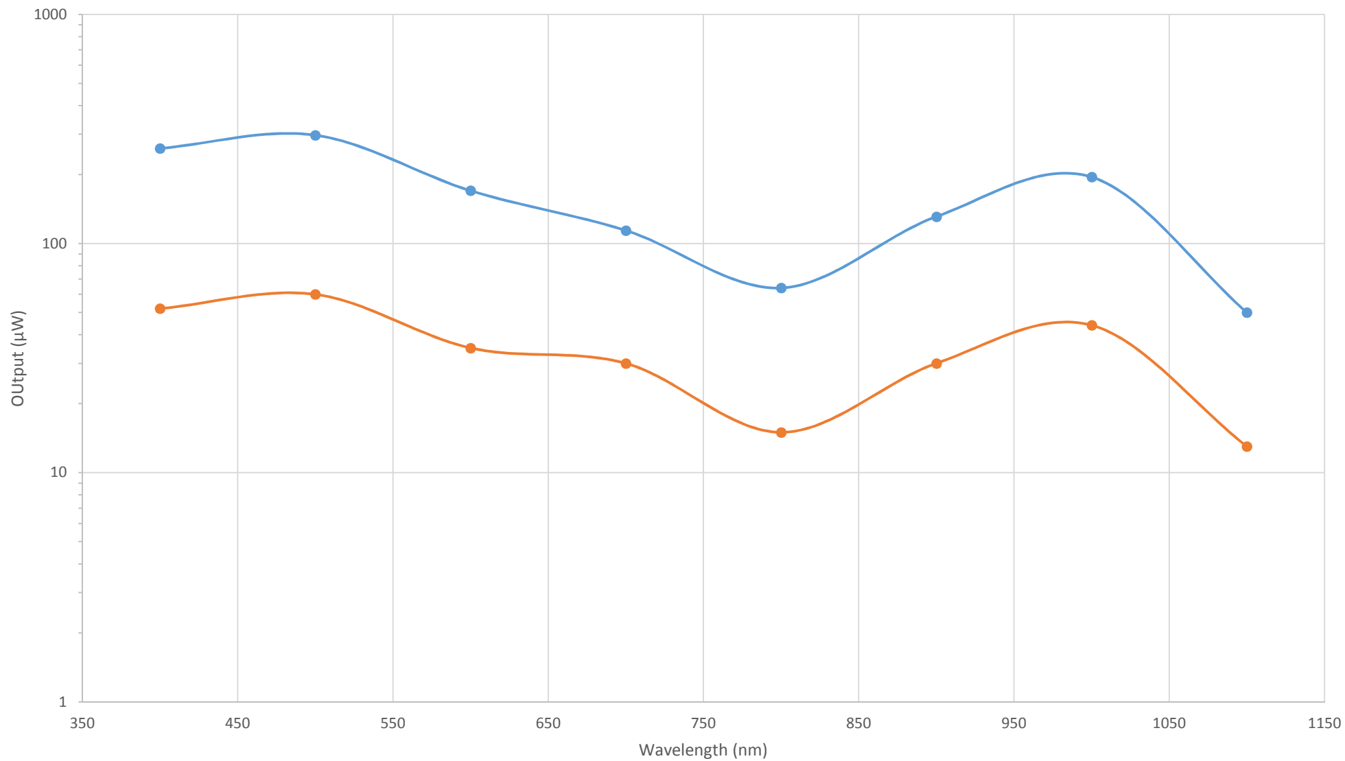
Output, 1200 lines/mm, blaze 400nm, slit
