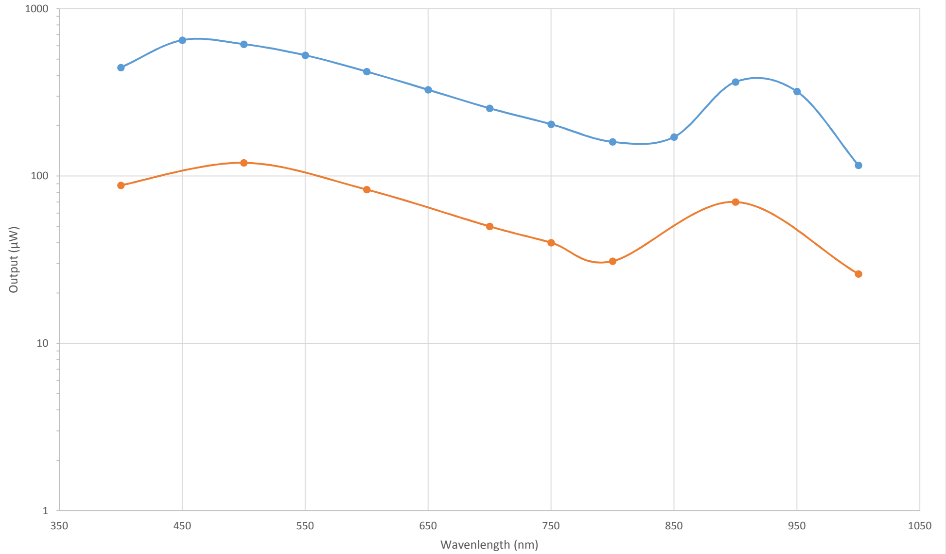
Output, 600 lines/ mm, blaze 500nm, slit
