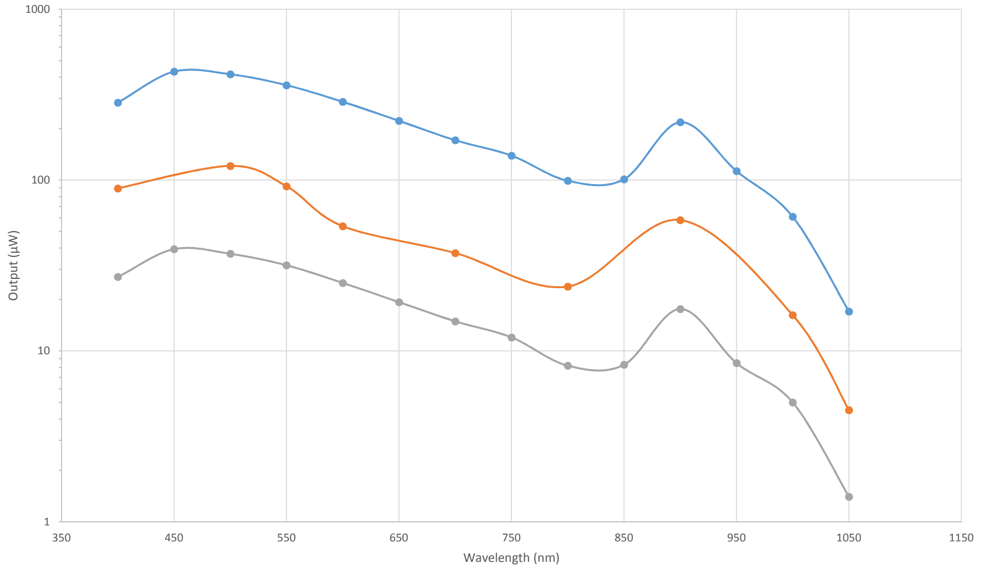
Output, 600 lines/ mm, blaze 500nm, fiber
